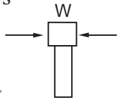
C6 Carbide tipped BRAZED V-GROOVE TIP 8°
