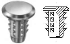
RAMPA Knock-in Inserts type TSLZ
